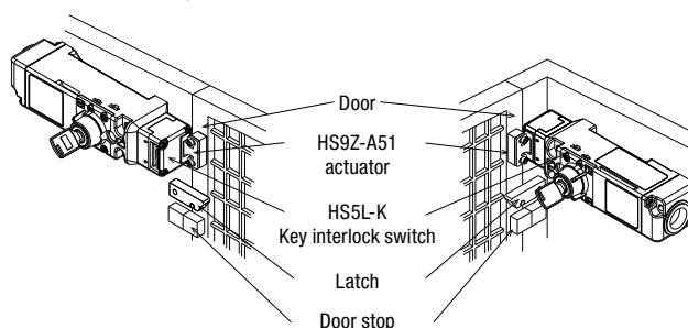
Application on sliding doors
