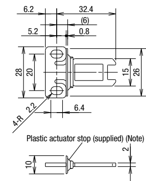
Actuator mounting hole layout (Straight actuator, right-angle actuator)
