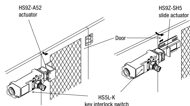
Application on hinged doors
