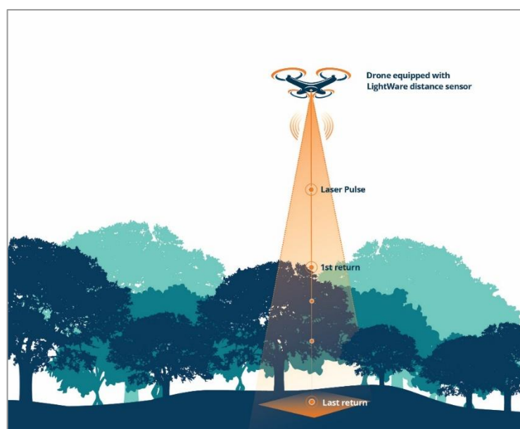
Figure 22: First and last pulse detection
