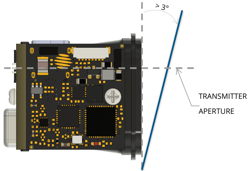
Figure 19: Behind-glass installation angle
