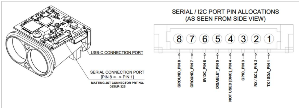
Figure 21: Communication cable pinout
