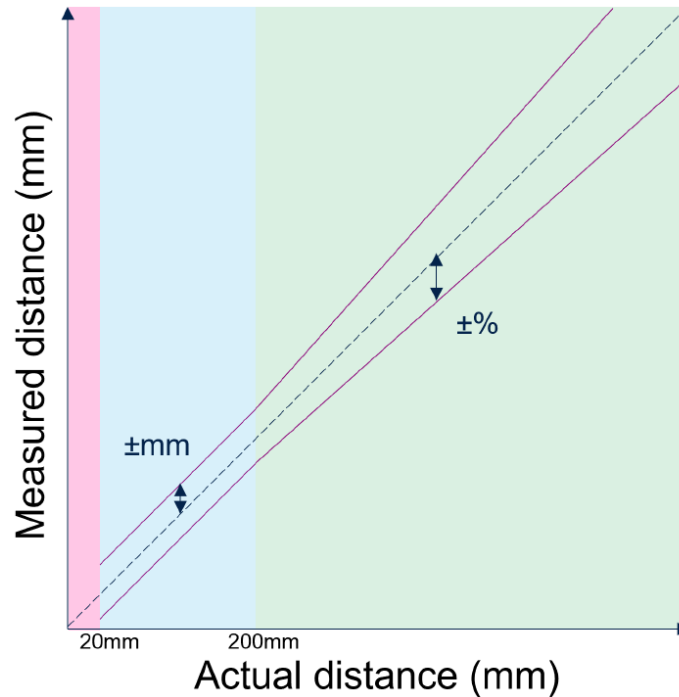
Figure 28. Range accuracy vs distance
