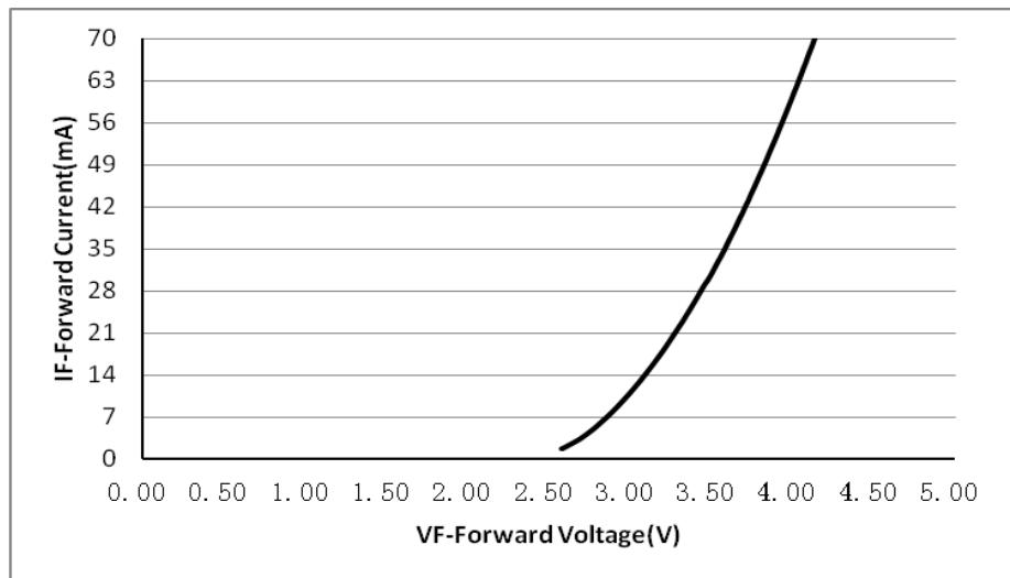
Figure1. Forward Current VS. Forward Voltage
