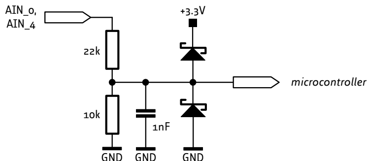
Figure 3.10 General purpose analog input circuit
