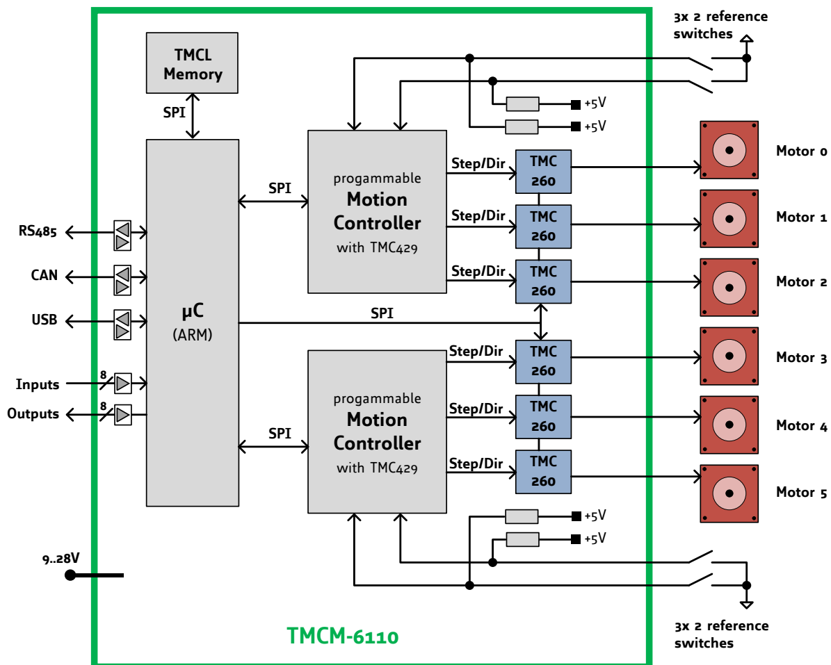
Figure 7.1: TMC6110 block diagram
