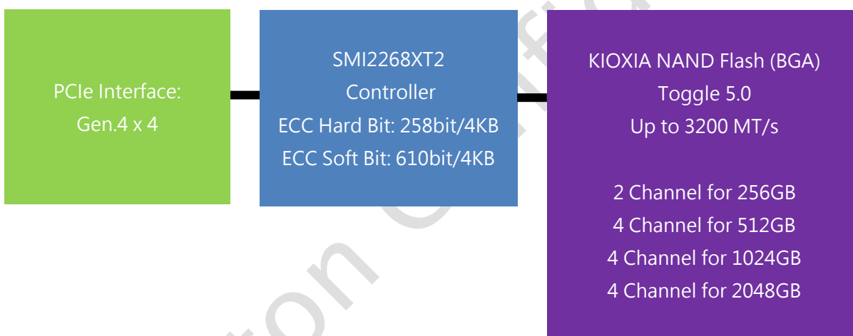
Fig 1-1: Kingston SSD OM8SGP4 Block Diagram
