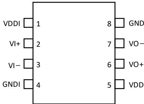
Figure 2. Si82B40x Pinout
