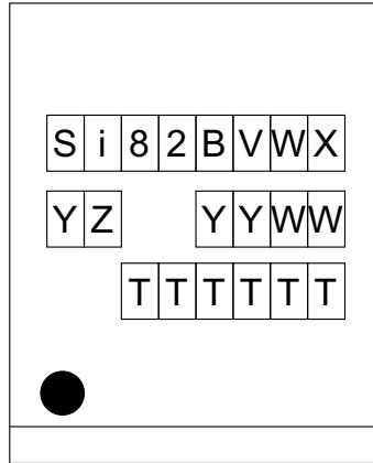
Figure 50. 8-Pin Wide Body SOIC (SSO) Top Marking
