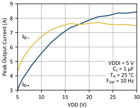
Figure 33. Peak Output Current vs. Gate Driver Supply Voltage
