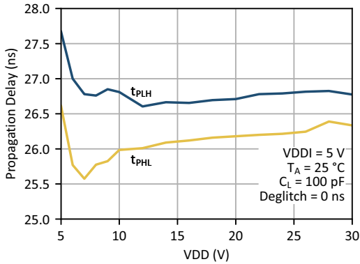
Figure 23. Propagation Delay vs. Gate Driver Supply Voltage
