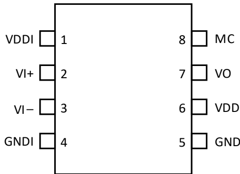
Figure 5. Si82B44x Pinout
