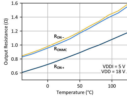
Figure 42. Output Resistance vs. Ambient Temperature
