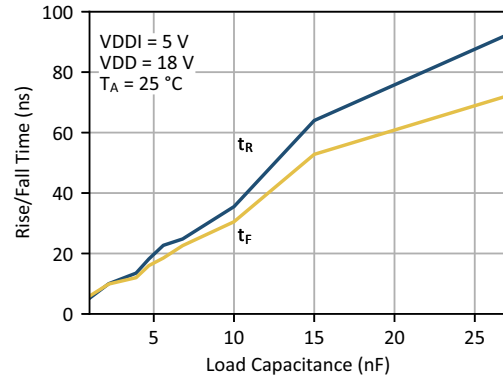
Figure 32. Output Rise/Fall Time vs. Output Load
