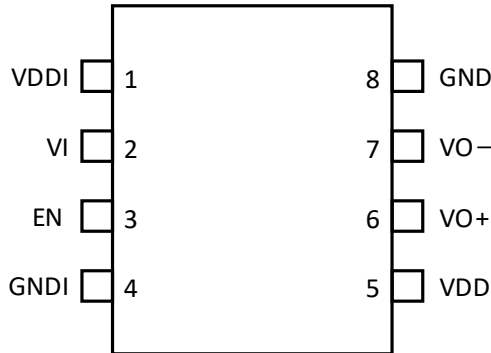
Figure 1. Si82B30x Pinout
