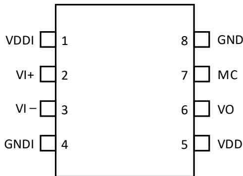
Figure 10. Si82B41x Pinout
