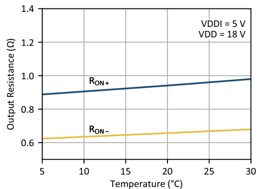
Figure 36. Output Resistance vs. Ambient Temperature
