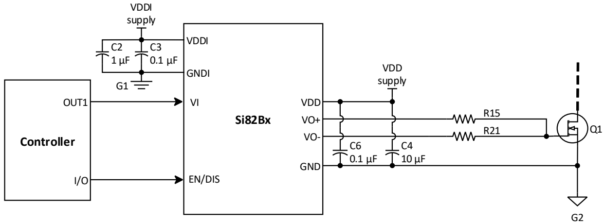
Figure 19. Si82Bx Split Output Application
