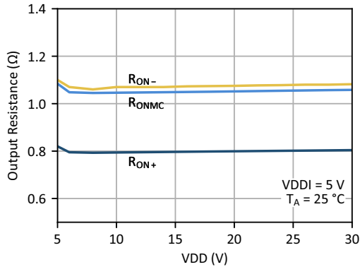
Figure 41. Output Resistance vs. Gate Driver Supply Voltage
