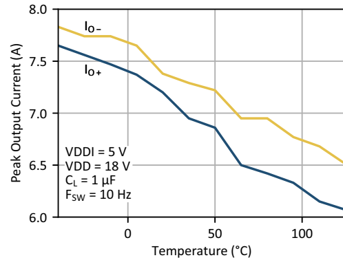
Figure 34. Output Current vs. Ambient Temperature
