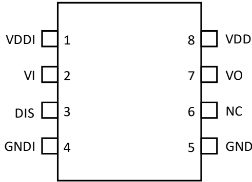
Figure 7. Si82B28x Pinout
