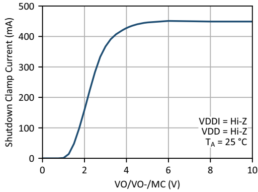
Figure 29. Shutdown Clamp Current vs. Shutdown Clamp Voltage
