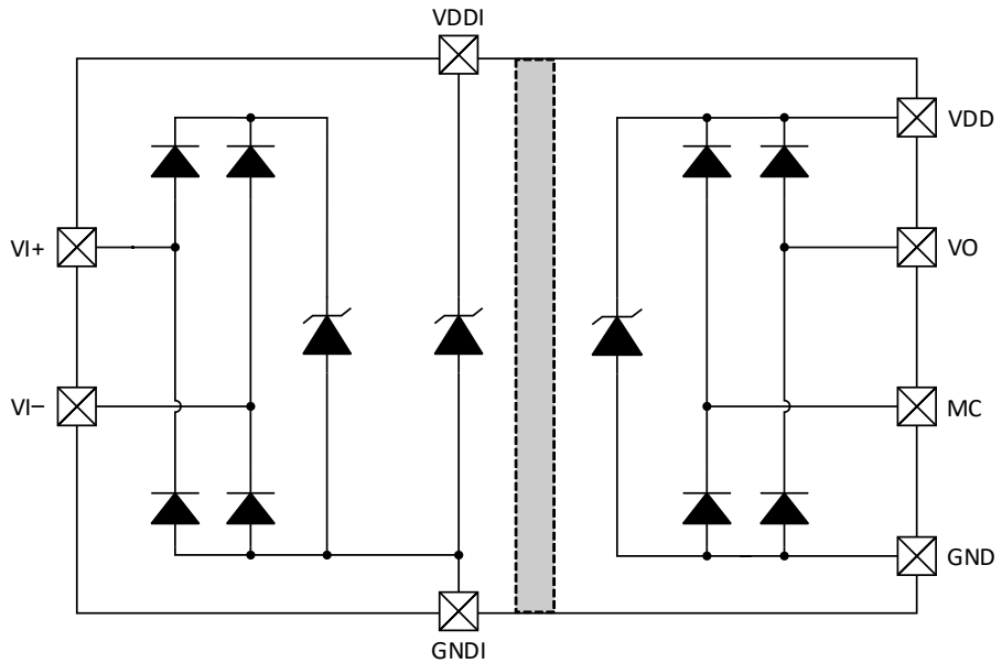
Figure 17. Si82B41x/44x/47x Device ESD Structure
