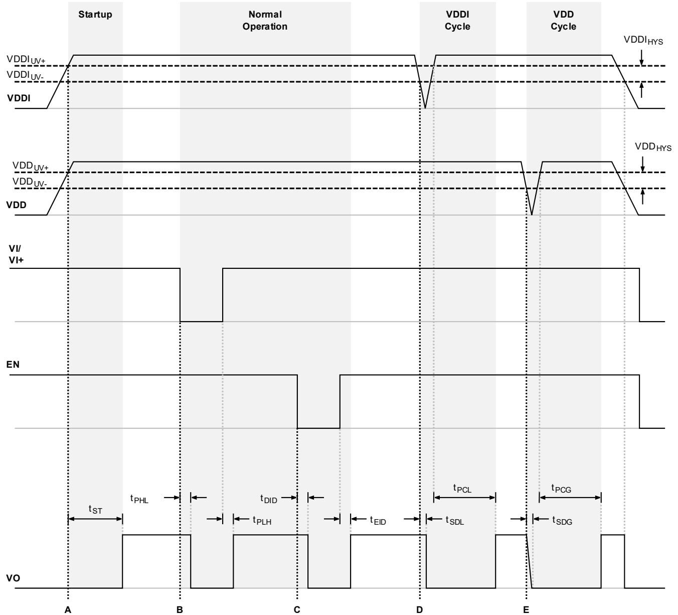
Figure 14. Gate Driver Timing Behavior
