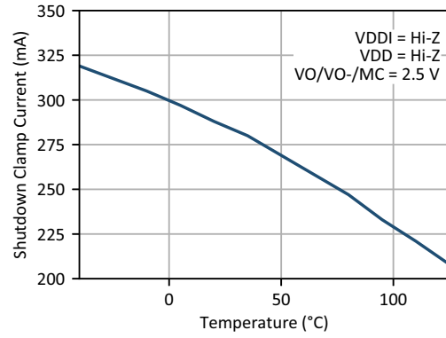
Figure 30. Shutdown Clamp Current vs. Ambient Temperature
