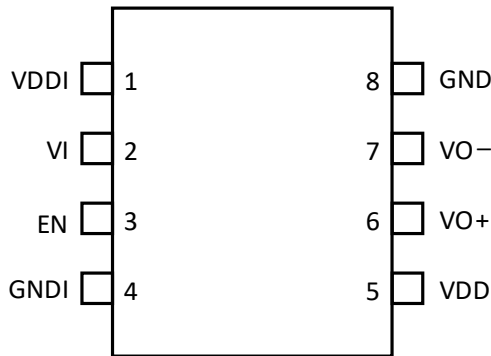
Figure 8. Si82B30x Pinout
