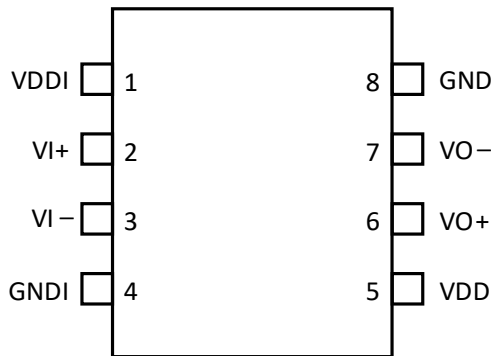
Figure 9. Si82B40x Pinout
