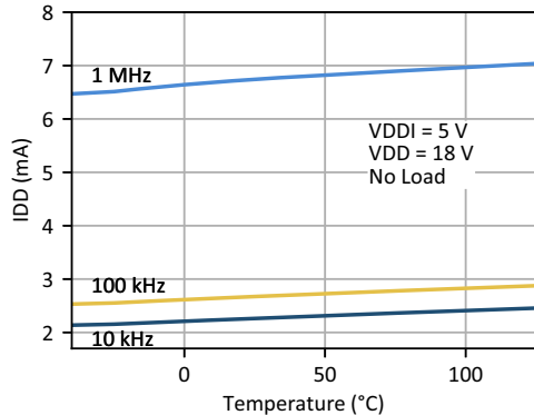
Figure 28. Gate Driver Active Supply Current vs. Ambient Temperature
