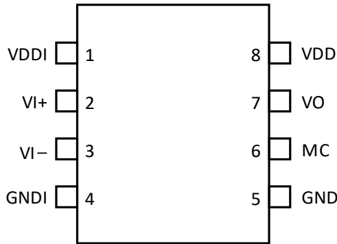
Figure 6. Si82B47x Pinout
