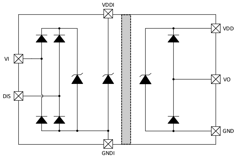
Figure 15. Si82B28x Device ESD Structure
