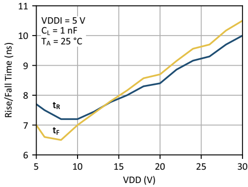
Figure 31. Output Rise/Fall Time vs. Gate Driver Supply Voltage
