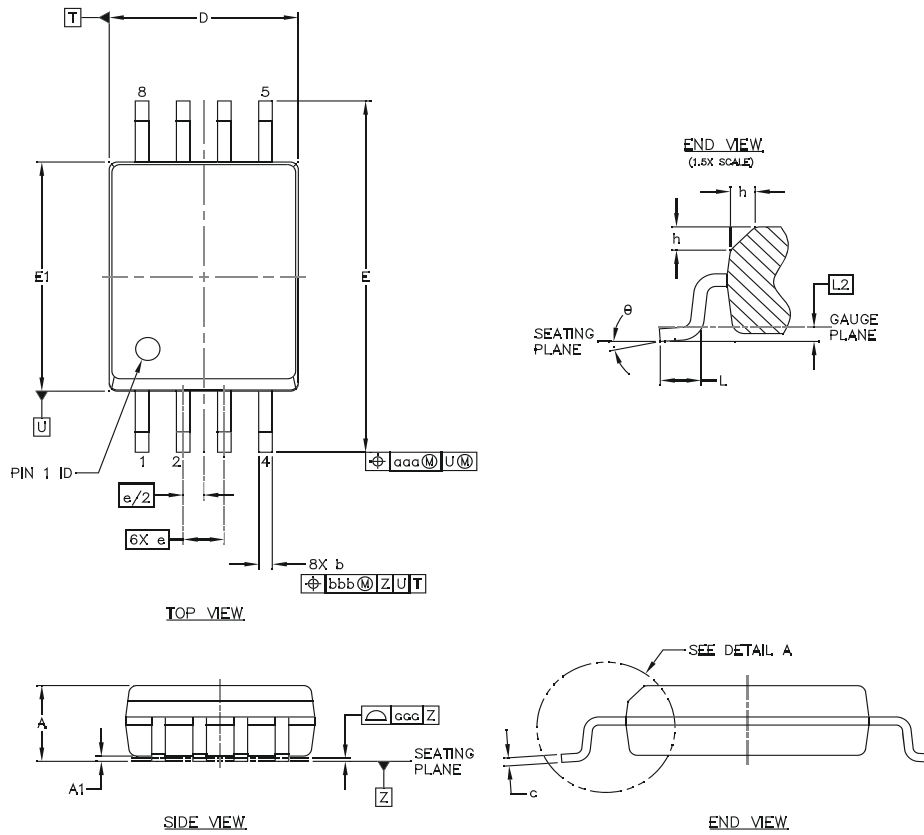
Figure 46. SSO-8 Package Drawing
