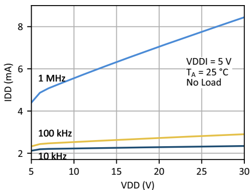
Figure 27. Gate Driver Active Supply Current vs. Gate Driver Supply Voltage
