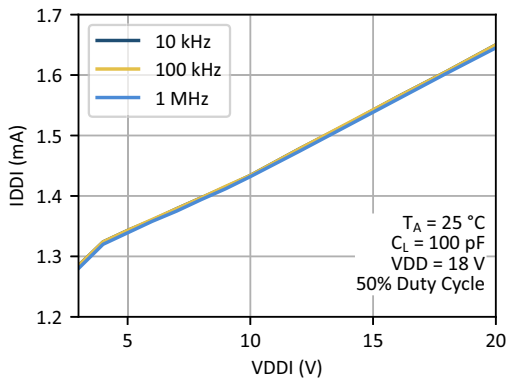
Figure 25. Logic Input Active Supply Current vs. Logic Input Supply Voltage
