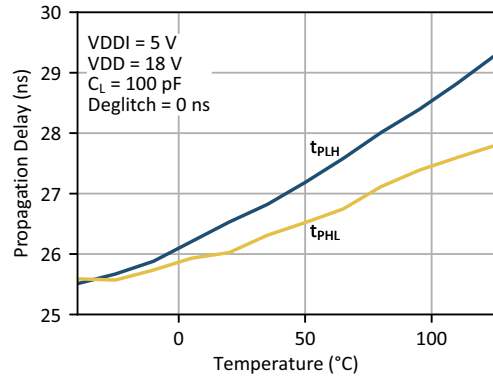
Figure 24. Propagation Delay vs. Ambient Temperature
