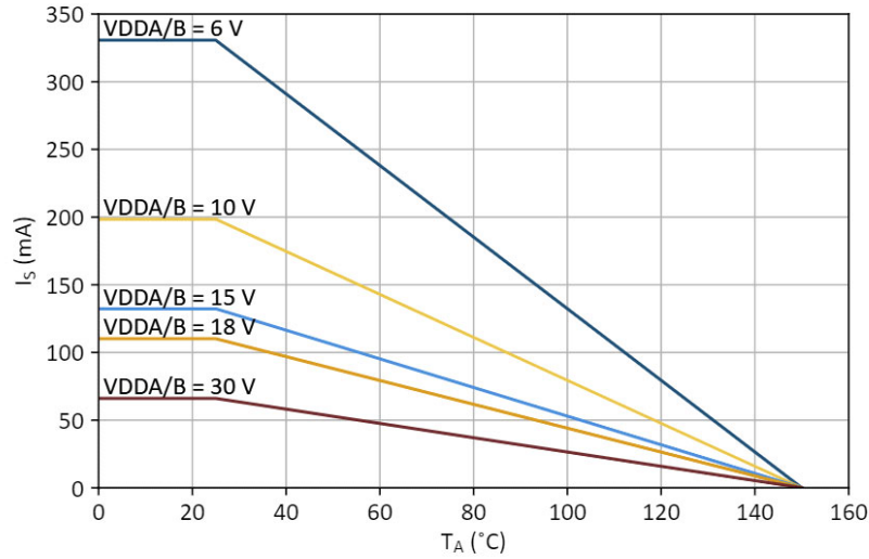
Figure 43. NB SOIC-8 Safety Current vs. Ambient Temperature Derating Curve
