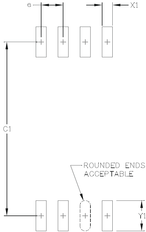
Figure 48. SSO-8 PCB Land Pattern
