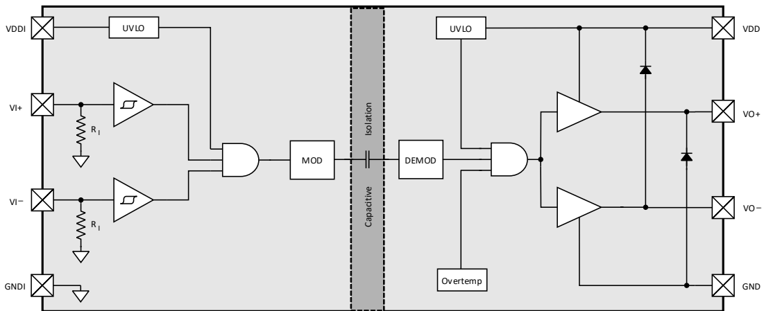
Figure 13. Si82B40x with Split Output and Complimentary Input
