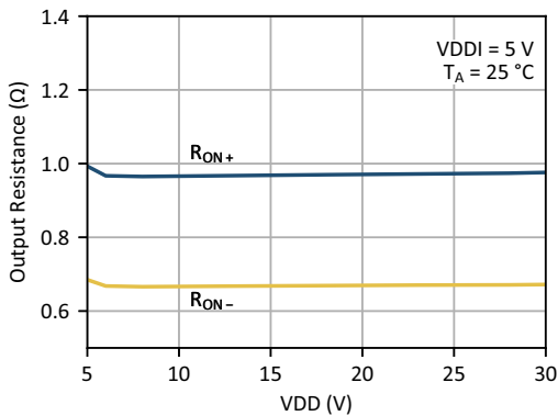
Figure 35. Output Resistance vs. Gate Driver Supply Voltage
