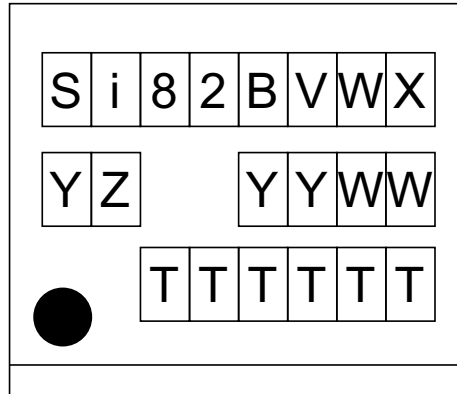
Figure 49. 8-Pin Narrow-Body SOIC Top Marking
