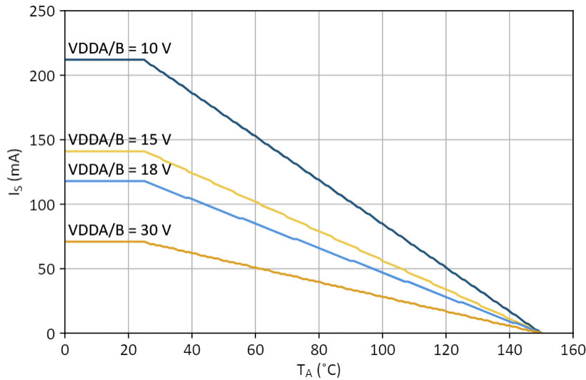
Figure 44. SSO-8 Safety Current vs. Ambient Temperature Derating Curve
