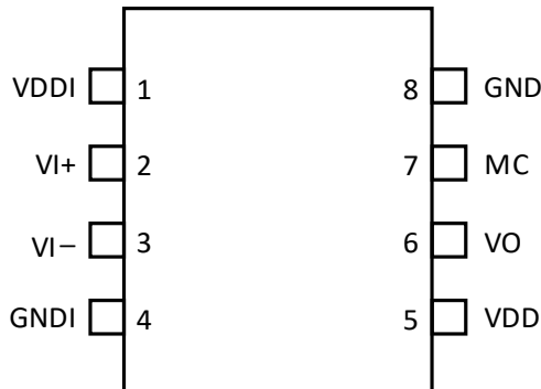
Figure 3. Si82B41x Pinout
