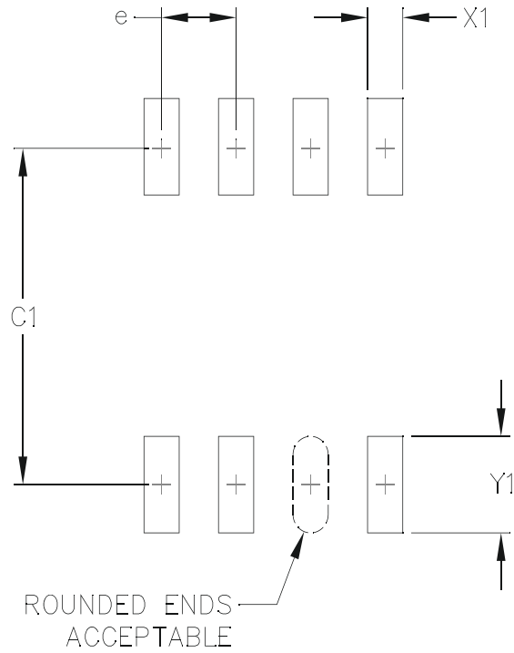
Figure 47. NB SOIC-8 Land Pattern
