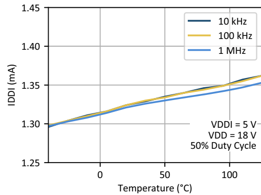
Figure 26. Logic Input Active Supply Current vs. Ambient Temperature
