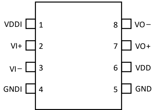
Figure 4. Si82B43x Pinout
