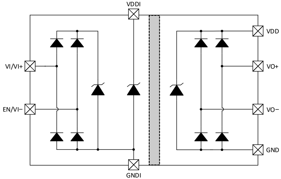
Figure 16. Si82B30x/40x/43x Device ESD Structure
