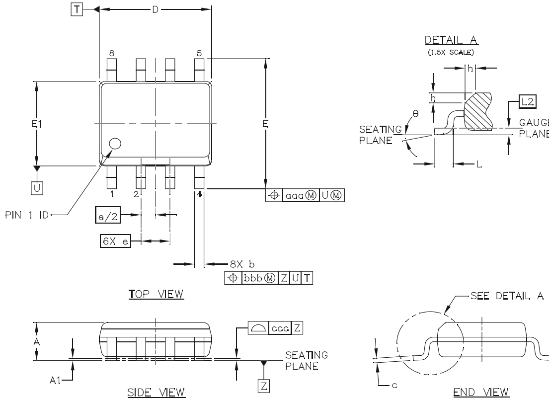
Figure 45. NB SOIC-8 Package Drawing
