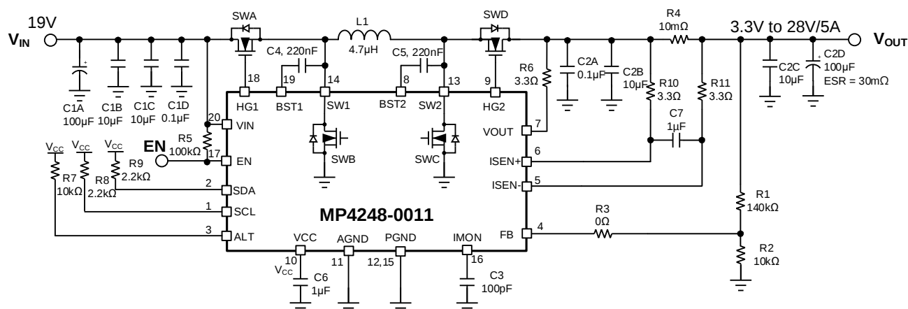
Figure 17: Typical Application Circuit ( V_{IN} = 19V , V_{OUT} = 3.3V to 28V/5A , 140W EPR Application) (11)
