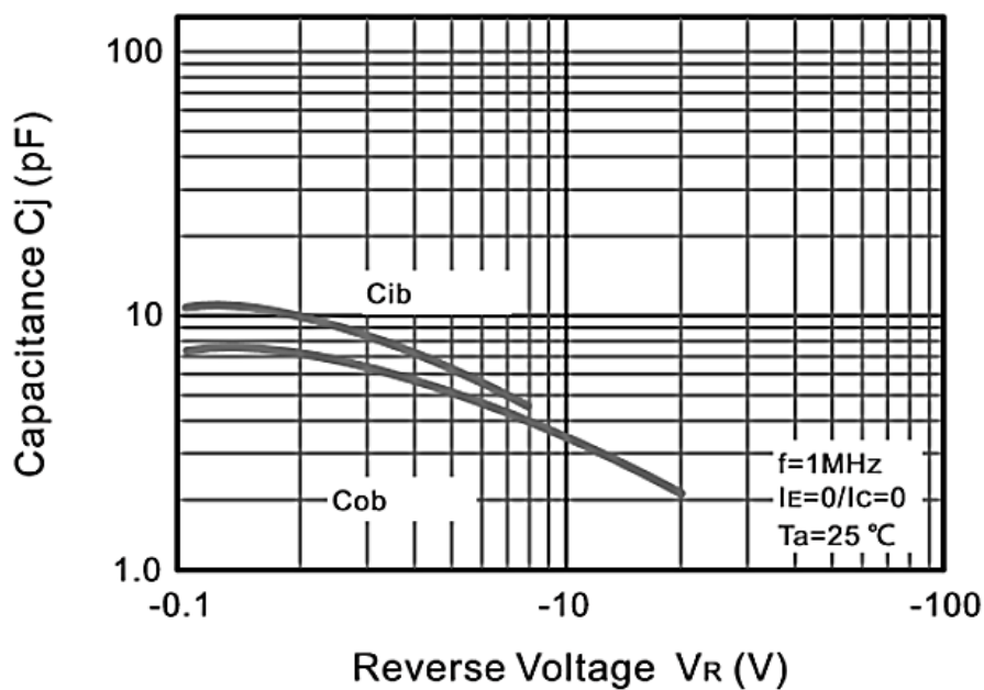
Fig.8 C_{ob}/C_{ib} -- V_{CB}/V_{EB}
