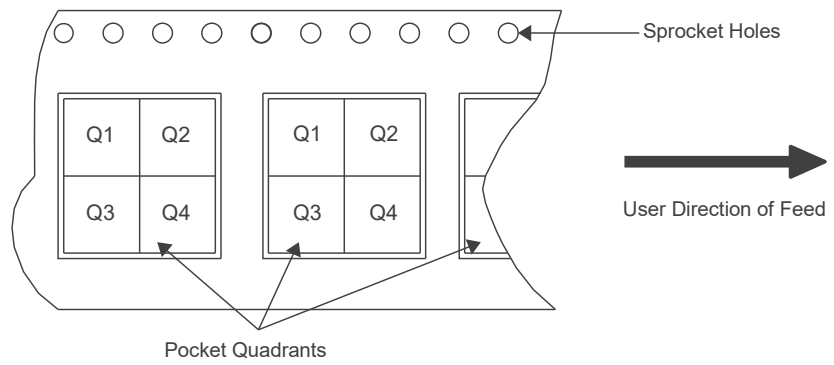
Figure 13.2: Tape and Reel Specification
