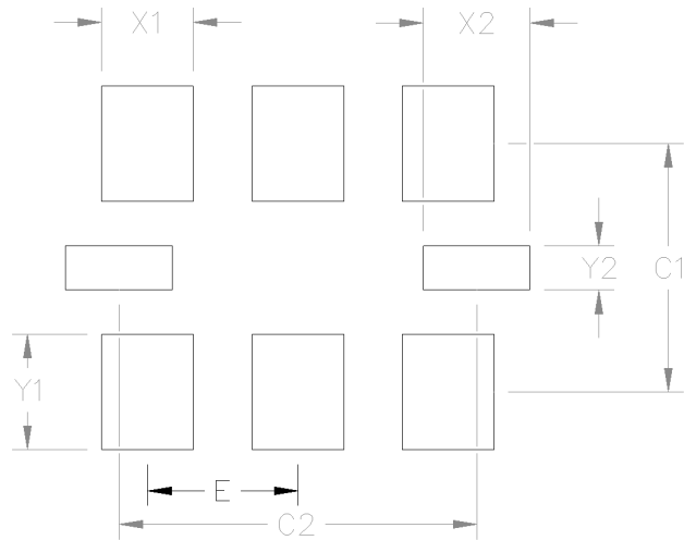
Figure 7.1. Si544 (5x7 mm) PCB Land Pattern
