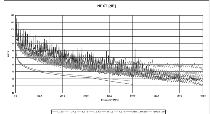
E-DAT modul Linkperformance 10 GBit Ethernet up to 100 m
