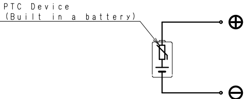
CIRCUIT DIAGRAM [回路図]
